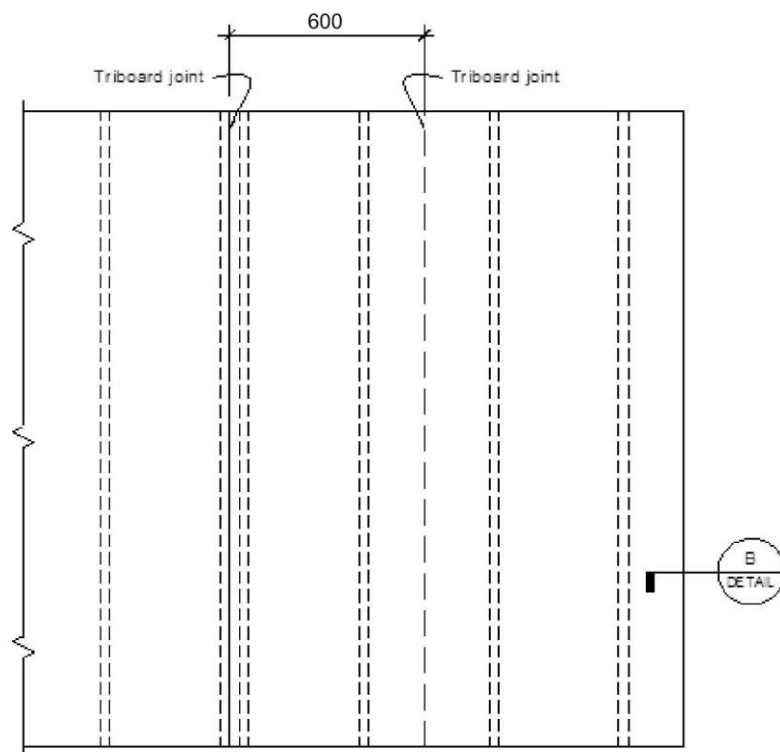
PANEL ELEVATION
