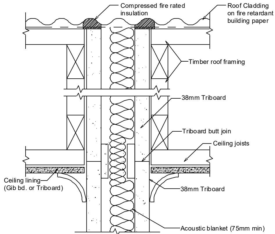
Timber Ceiling
