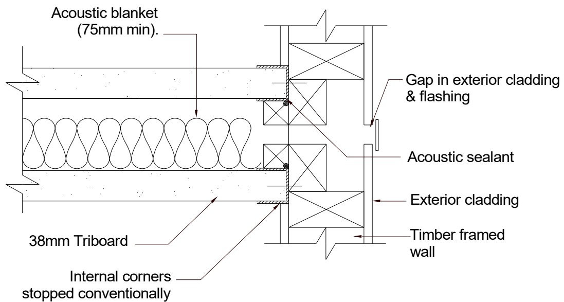
Timber Wall
