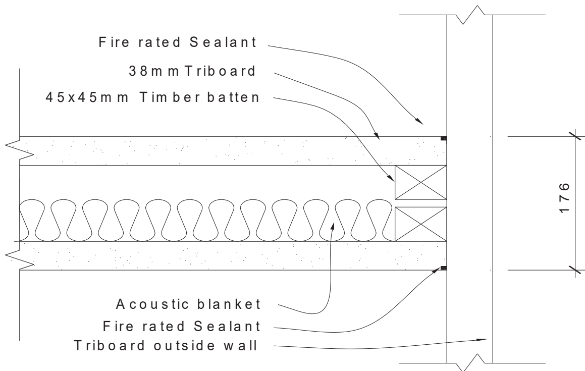
DETAIL B
