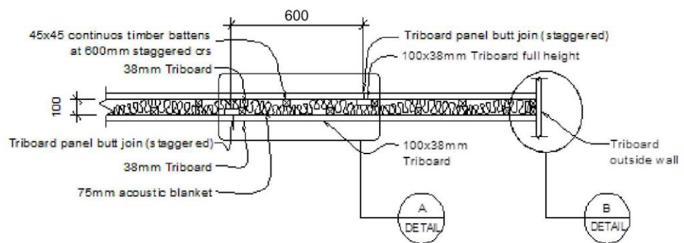
PLAN SECTION
