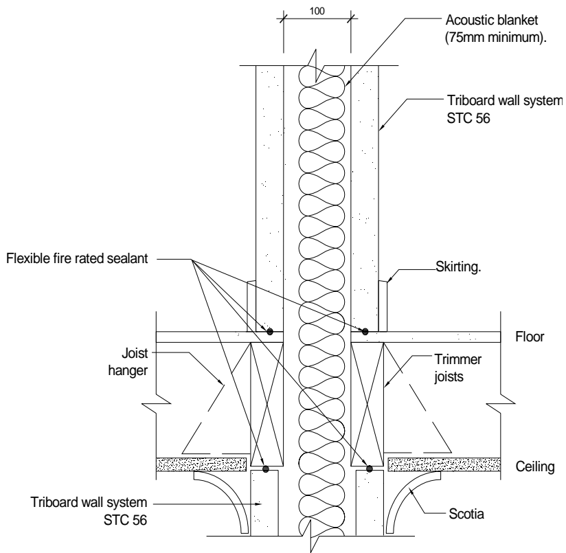
Wall / Floor Junction
