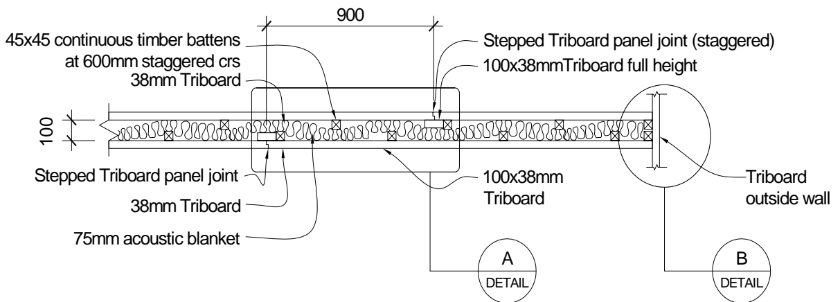
PLAN SECTION
